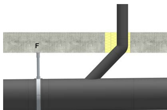
Figure 7.22 Creation of a fixed point on large diameter pipes using a double flange bushing (for HDPE).
