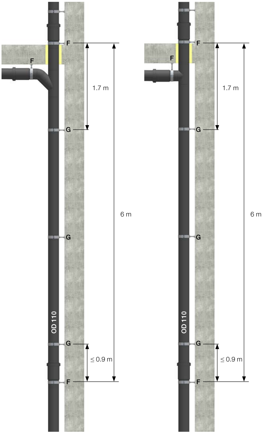
Connection with 45° branches
