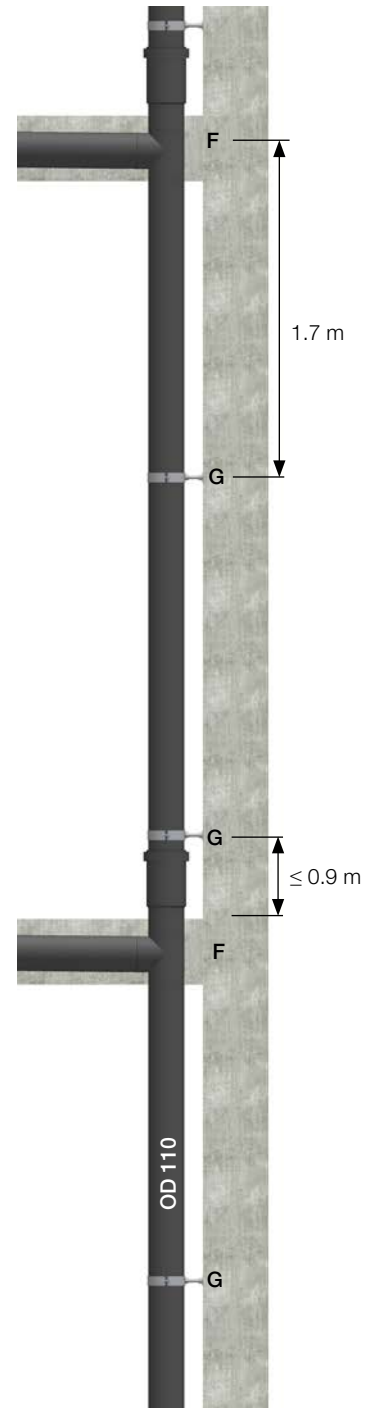
Figure 7.30 Stack OD=110 mm with inlet branches embedded in the slab (for HDPE).
